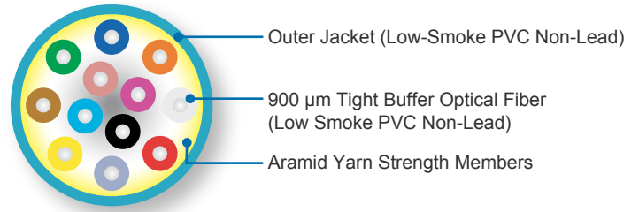
Single-Tube Cable Example: 12 Fibers or less with no central member
