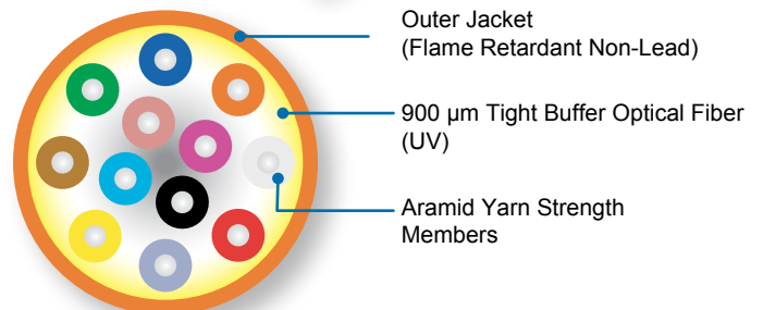
Single-Tube Cable Example: 12 Fibers or less with no central member
