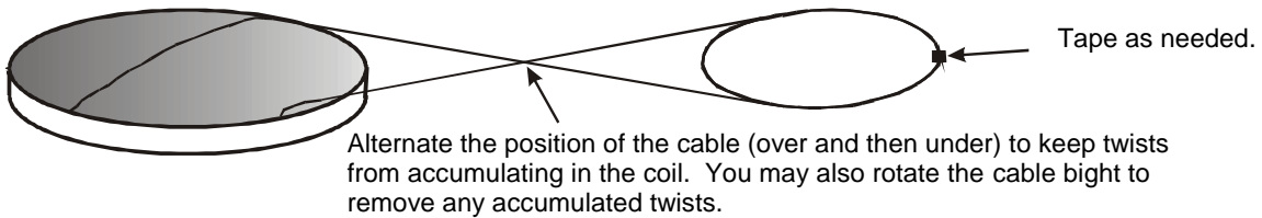
Figure 13 - Fold-Over Method
