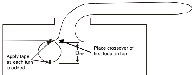
Step 2. Form the first turn in the cable. See Table 1 for the minimum storage-coil diameter ( D_{min} ).
