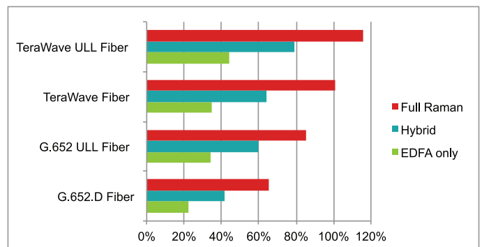
Expected regeneration distance at 400 G compared to standard single-mode fiber at 100 G using EDFA
