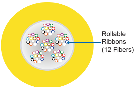
72-Fiber R-Pack RR Cable Cross-Section
