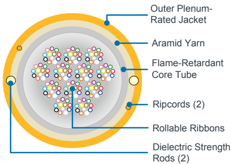
AccuFlex Rollable Ribbon Cable Cross-section
