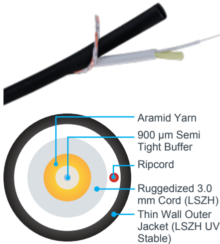
EZ-Peel 4.8 mm Drop Cable Cross-Section
