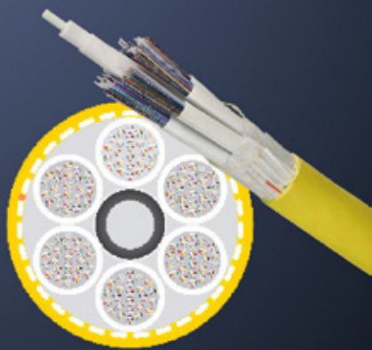
AccuTube RR I/O Cable 1728-Fiber Count
