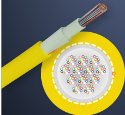
AccuRiser RR Cable 144-864-Fiber Count
