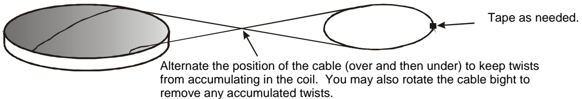
Figure 13 - Fold-Over Method
