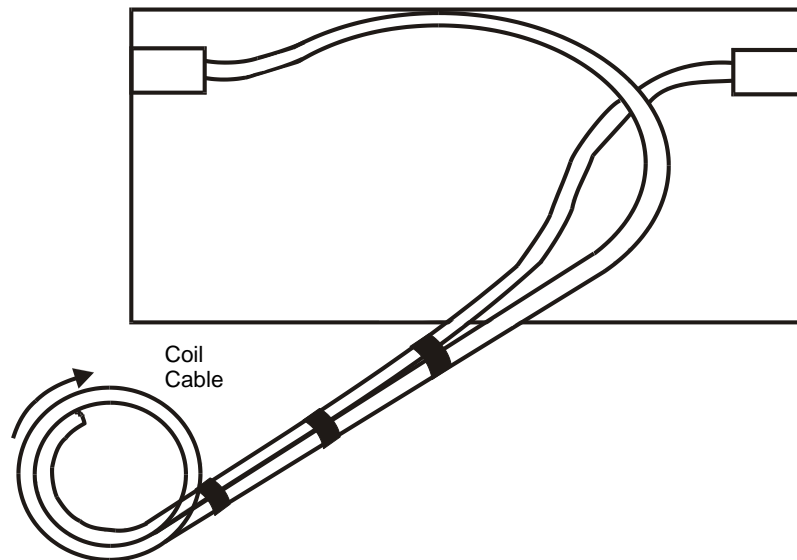
Figure 18 - Coiling cable slack at splice location.
