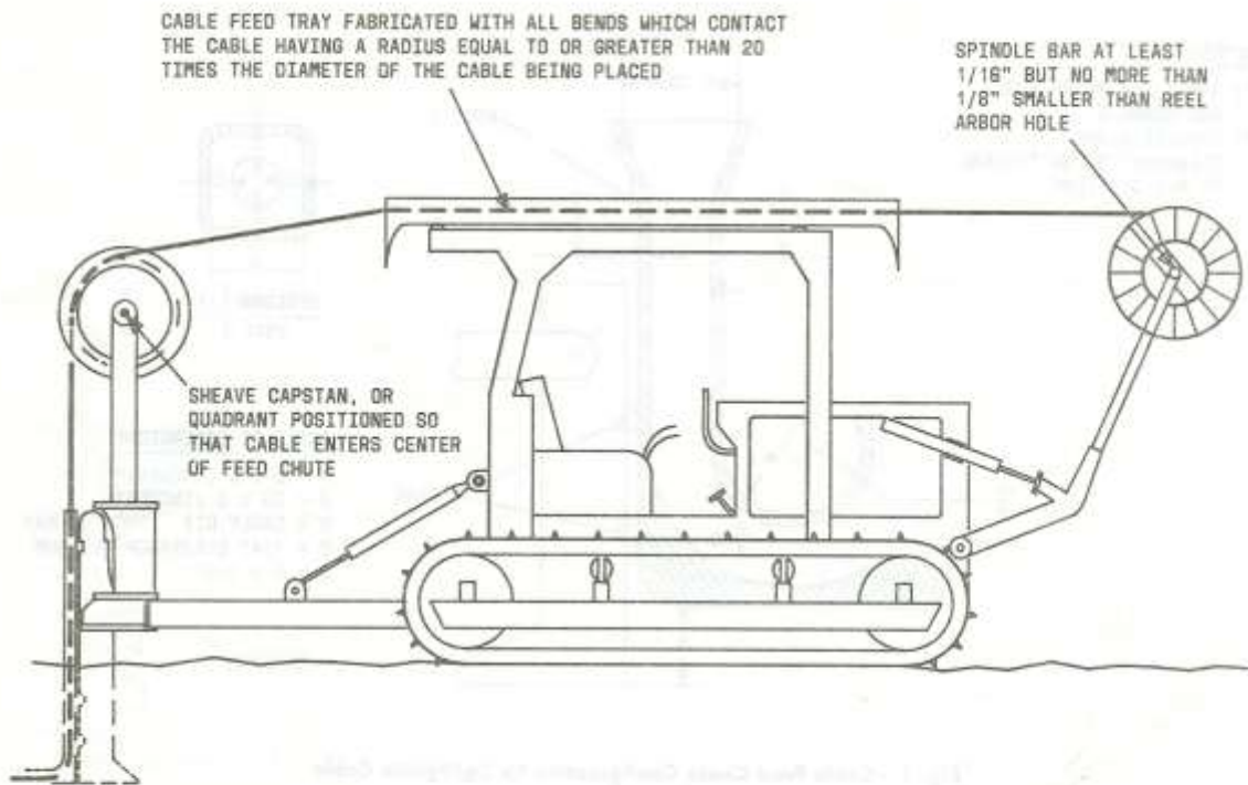
Fig. 1—Typical Cable Delivery System
