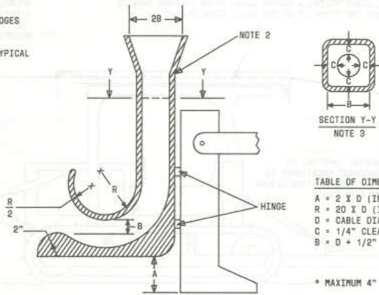
Fig. 2—Cable Feed Chute Configuration for Lightguide Cable
