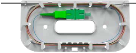
Internal view of Standard POE Module
