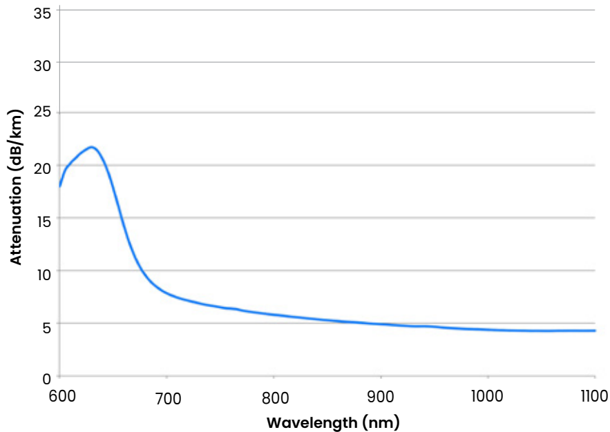
Typical Spectral Attenuation for HCL Optical Fiber
